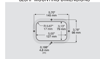
823RF MOUNTING DIMENSIONS
